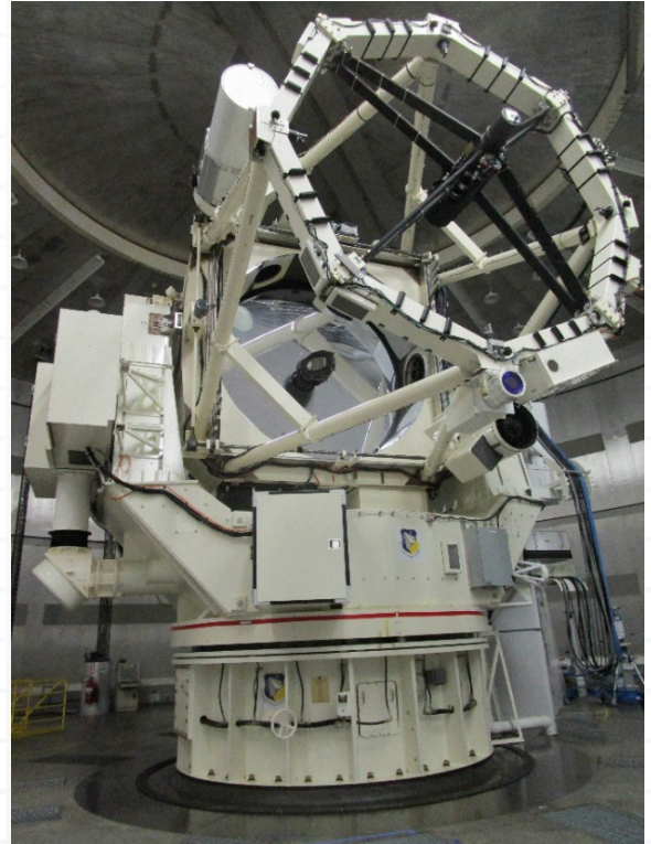
The 3.6-meter, 75-ton Advanced Electro-Optical System (AEOS) telescope shown above is the largest optical telescope in the Department of Defense. In addition the Maui Space Surveillance System facility houses several other telescopes ranging from 0.4 to 1.6-meters. Photo credit: AFRL
